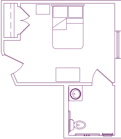
Standard Model
